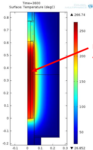
Conjugate heat transfer model
