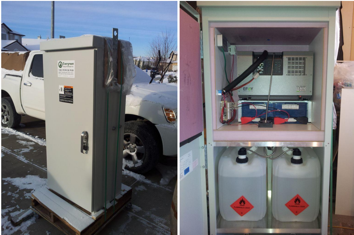
Latest Version of Power Pod (Type D) with CSA, improved exhaust, DuoCartSwitch, and (2) 28L Fuel Cartridges (61,600 Watt-hours of standby power)
